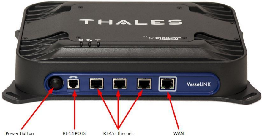
BDU Front Panel Detail
